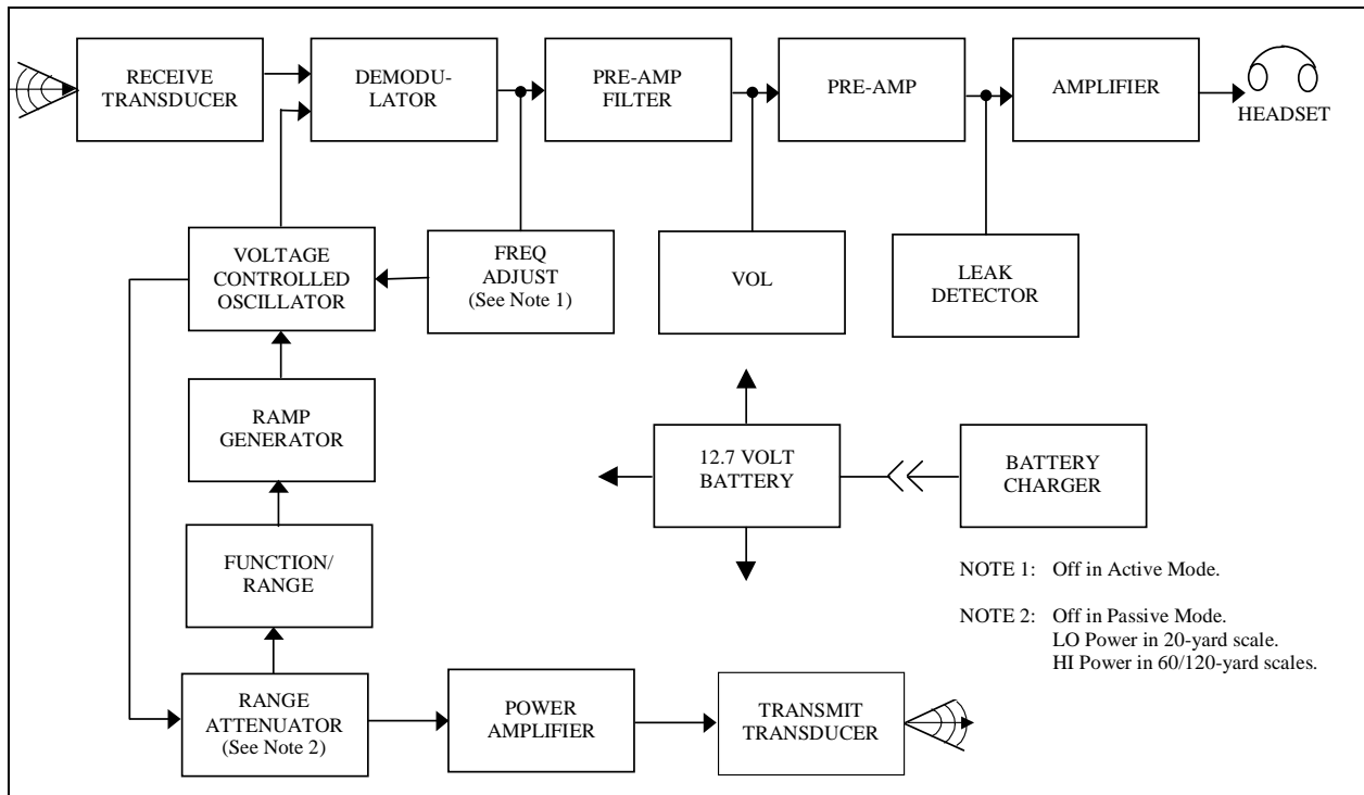
Figure 4 – DLS-2A Sonar Unit Functional Block Diagram
